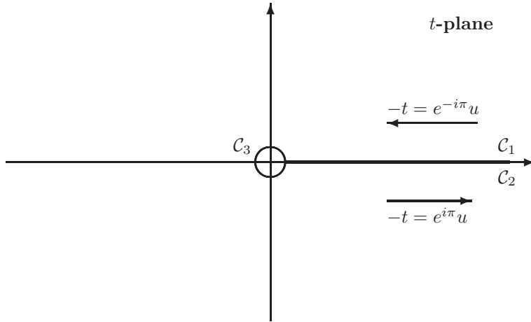
FIGURE 1. Contour \mathcal{C} in Lemma 2.6.
